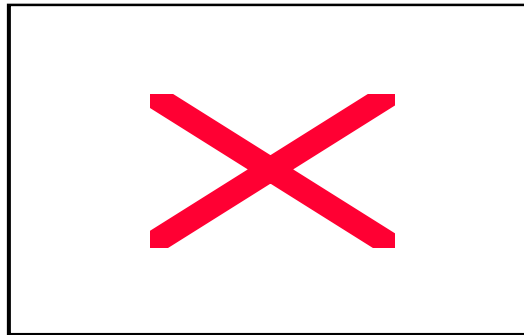
Figure 6.74 Draft
